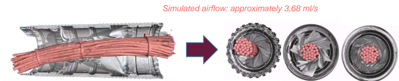
Fig. 6: Hilti Speed Sleeve CP 653 / CFS-SL with closing mechanism to increase air tightness – third-party CFD simulation by Paul Scherrer Institute from June 2016
